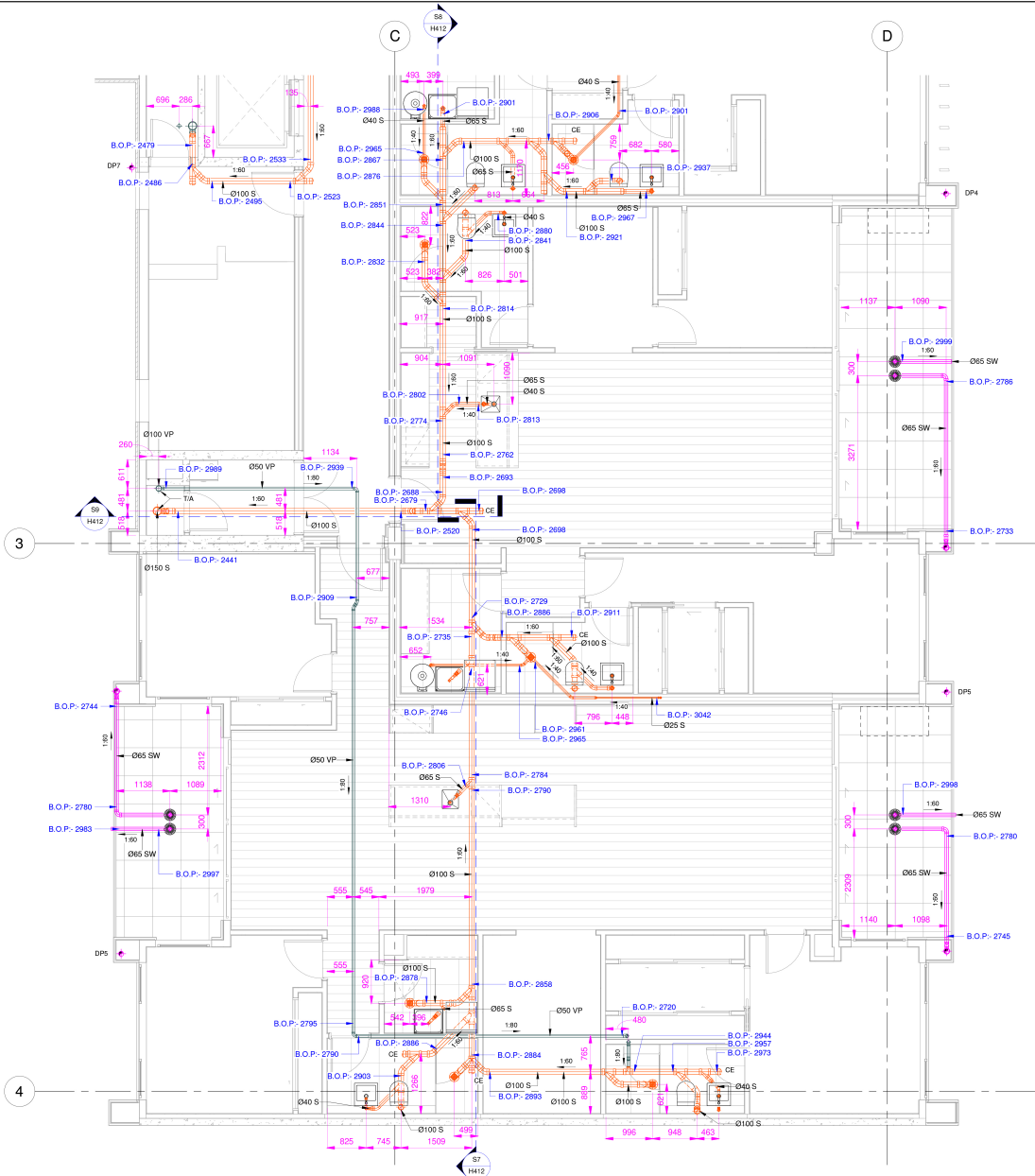
1 LEVEL 4 HIGH LEVEL SANITARY LAYOUT - PART 2 H412 1:50
