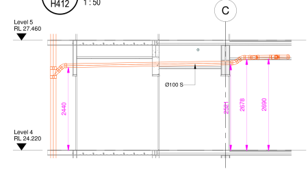
S9 SECTION L4-S9 H412 1:50
