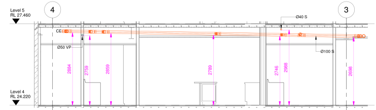
S7 SECTION L4-S7 H412 1:50
