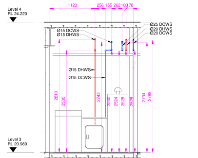
S21 SECTION L3-S21 H319 1:30
