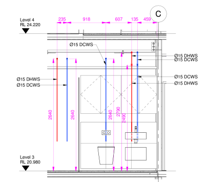
S22 SECTION L3-S22 H319 1:30
