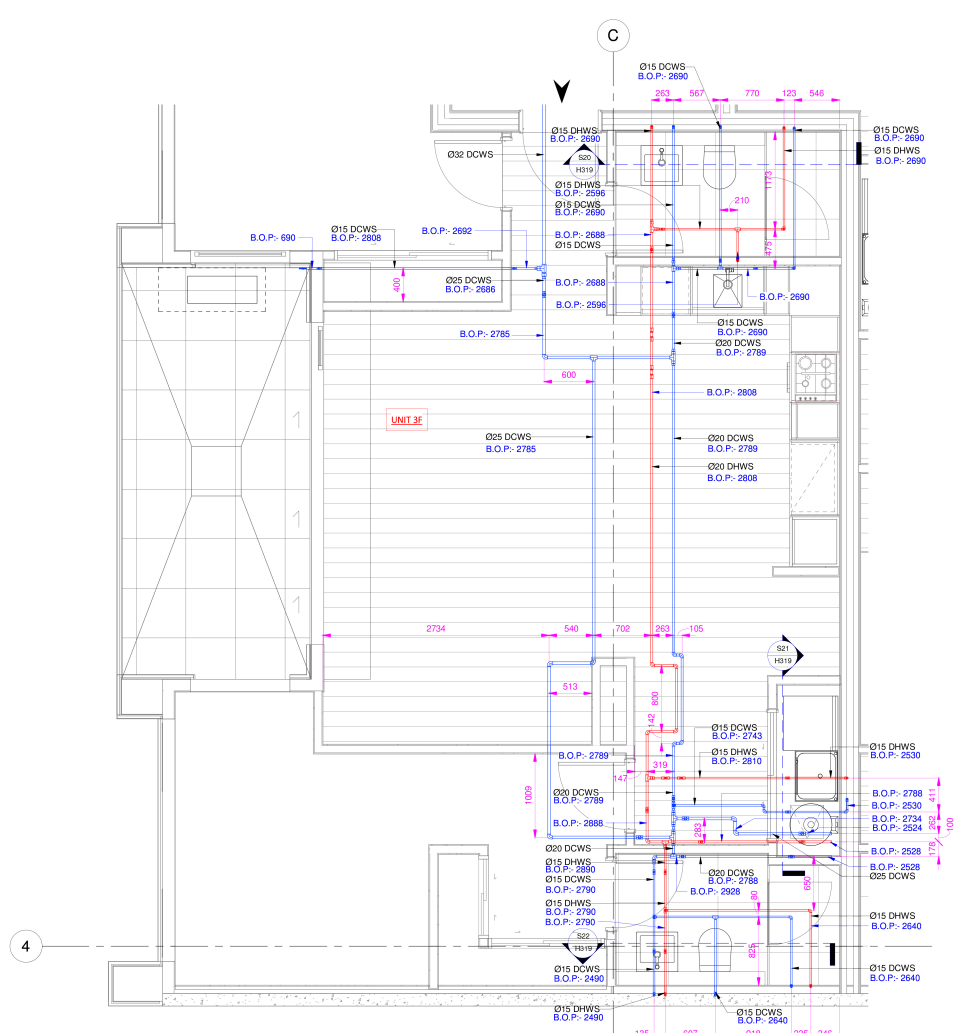
1 UNIT 3F WATER SUPPLY LAYOUT H319 1:30
