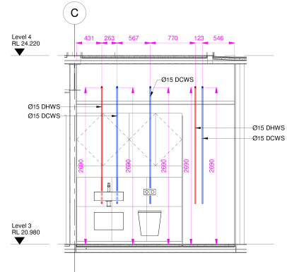
S20 SECTION L3-S20 H319 1:30
