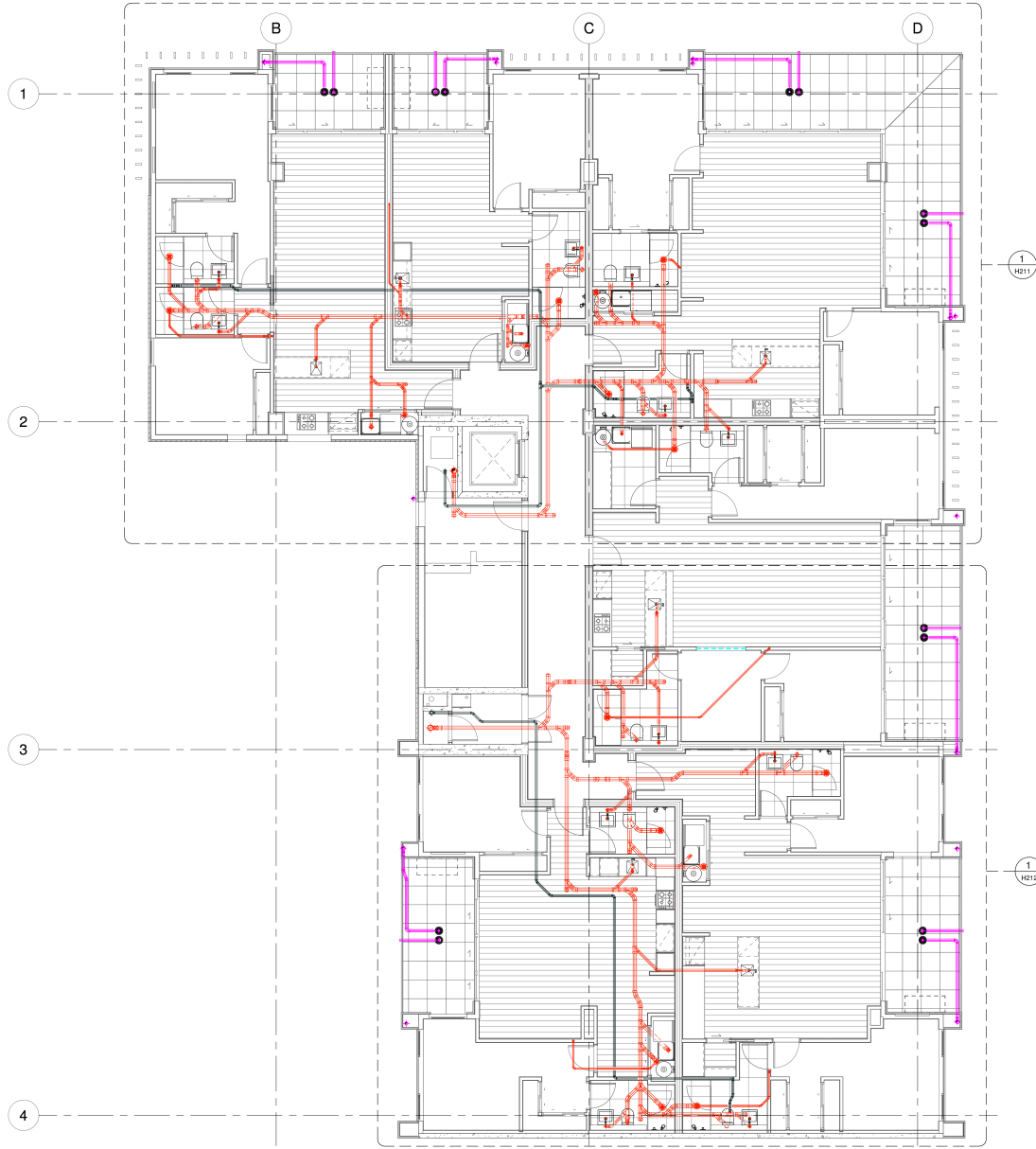
1 LEVEL 2 HIGH LEVEL SANITARY LAYOUT H201A 1:75
