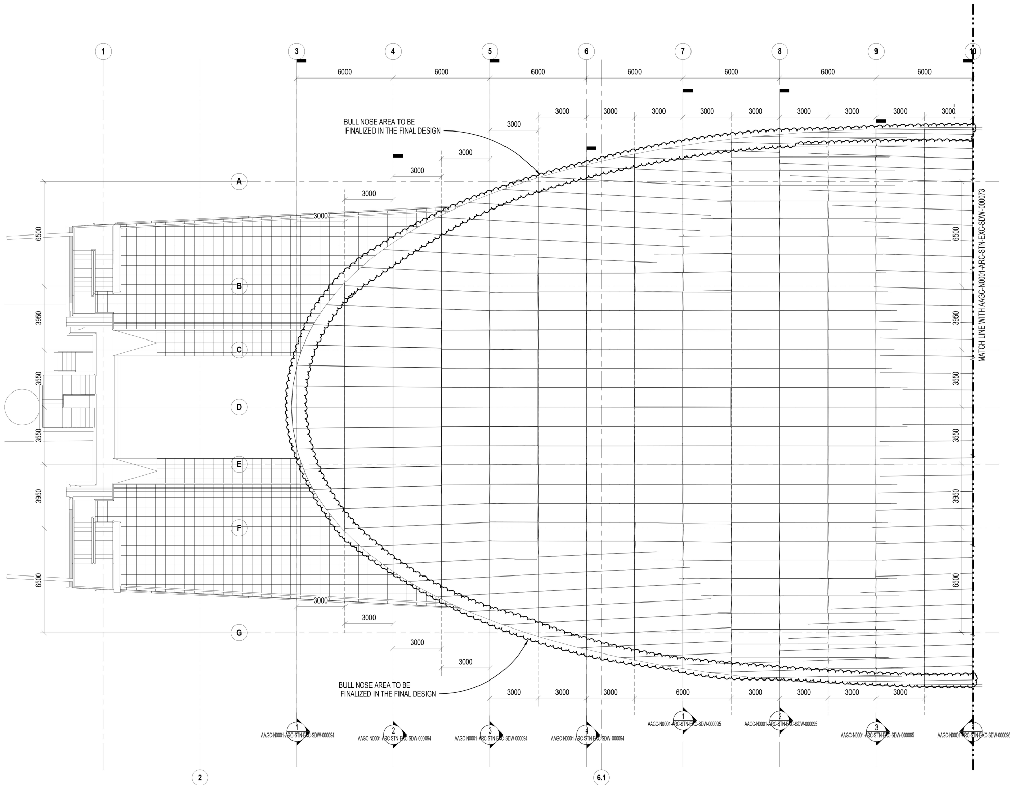
1 PART PLAN - 2 (FOR SOLID ALUMINUM CLADDING PANEL SUPPORT FRAMING LAYOUT) AAGC-N0001-ARC-STN-EXC-SDW-000073 SCALE 1 : 100
