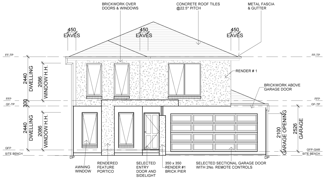
ELEVATION A SCALE 1 : 100 3.1
