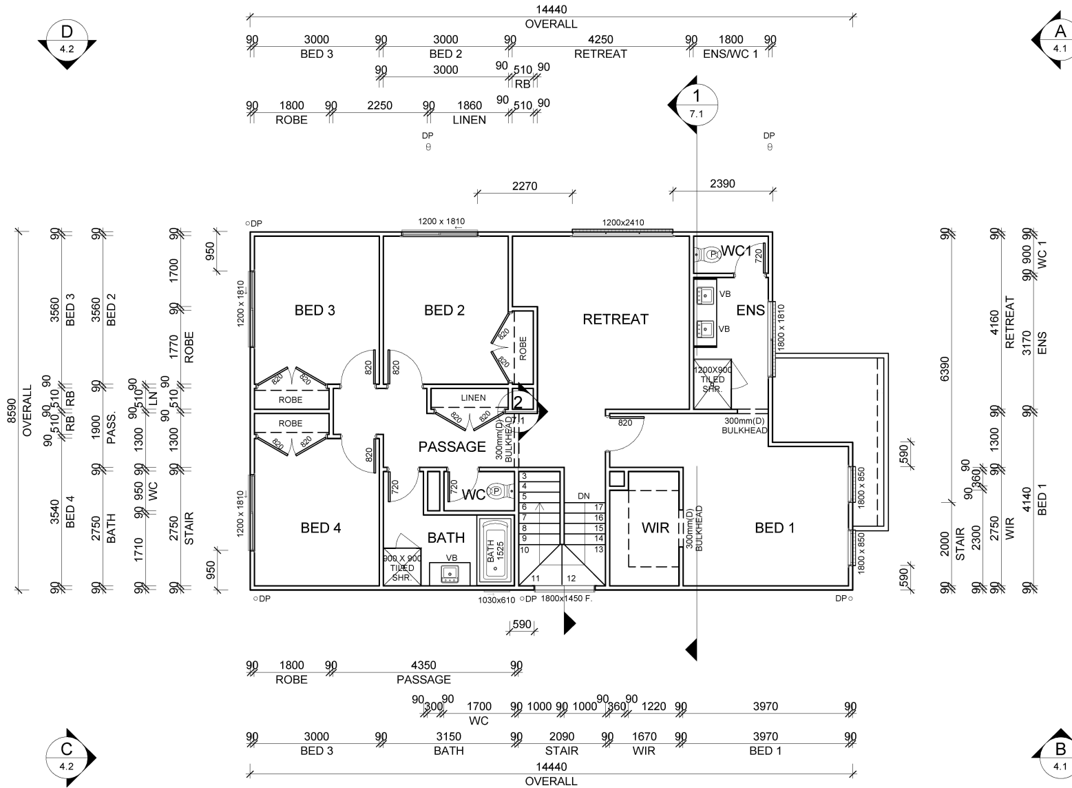
PLAN-FIRST FLOOR SCALE 1 : 100
