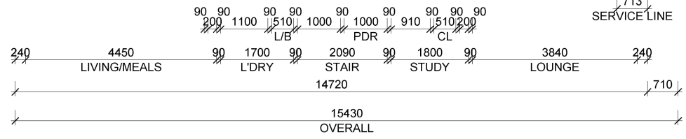
PLAN-GROUND FLOOR SCALE 1 : 100
