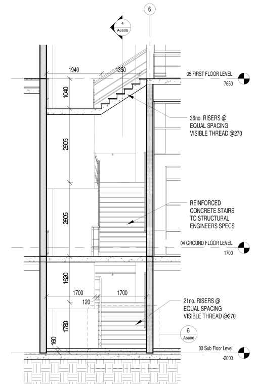
5 STAIR - 4 - CROSS SECTION 1:50
