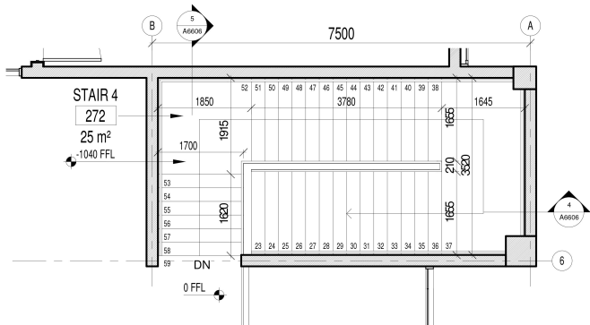
3 STAIR 4 - FIRST FLOOR PLAN 1:50
