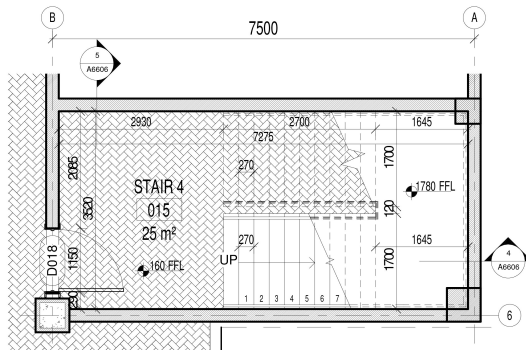
1 STAIR 4 - BASEMENT PLAN 1:50
