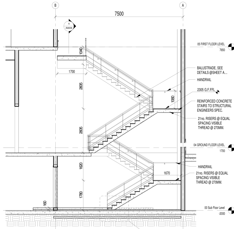
4 STAIR - 4 SECTION 1:50
