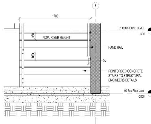
6 STAIR - 4 CROSS SECTION DETAIL 1:20
