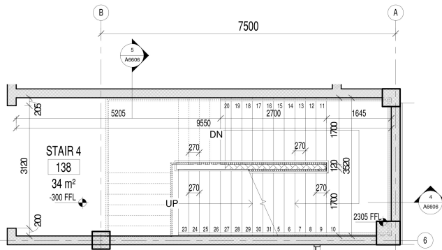
2 STAIR 4 - GROUND FLOOR PLAN 1:50
