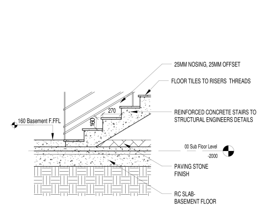
7 STAIR - 4 SECTION DETAIL 1:20
